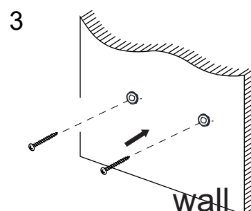
Tighten the screw to 5mm away from the wall
